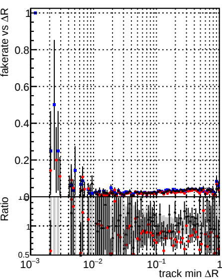
Fake rate vs \Delta R(\text{track, jet}) Legend: DQM TT original (blue squares) DQM TT mod modelsdeep_truthfinal_reg_modelTEST-24 (red circles) DQM TT mod modelsdeep_something3 (black triangles)
