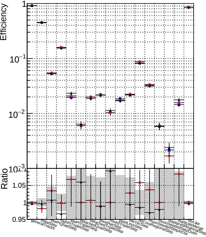
DQM_TT_original DQM_TT_mod_modelsdeep_truthfinal_reg_modelTEST-24 DQM_TT_mod_modelsdeep_something3
