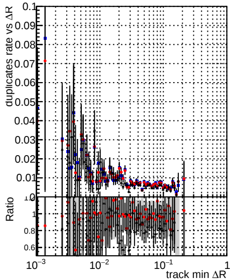
Legend for the top row of plots: \blacksquare DQM TT original \bullet DQM TT mod modelsdeep_truthfinal_reg_modelTEST-24 \blacktriangle DQM TT mod modelsdeep_something3
