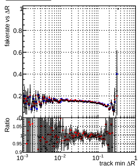
Legend: - \text{DQM\_TT\_original} (black line with dots) - \text{DQM\_TT\_mod\_modelsdeep\_truthfinal\_reg\_modelTEST-24} (red line with dots) - \text{DQM\_TT\_mod\_modelsdeep\_something3} (blue line with dots)
