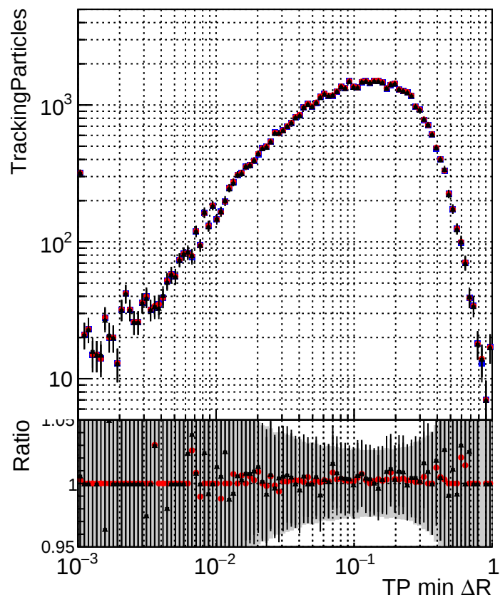
N of simulated tracks DQM TT original DQM TT mod modelsdeep truthfinal_reg_modelTEST-24 DQM TT mod modelsdeep something3
