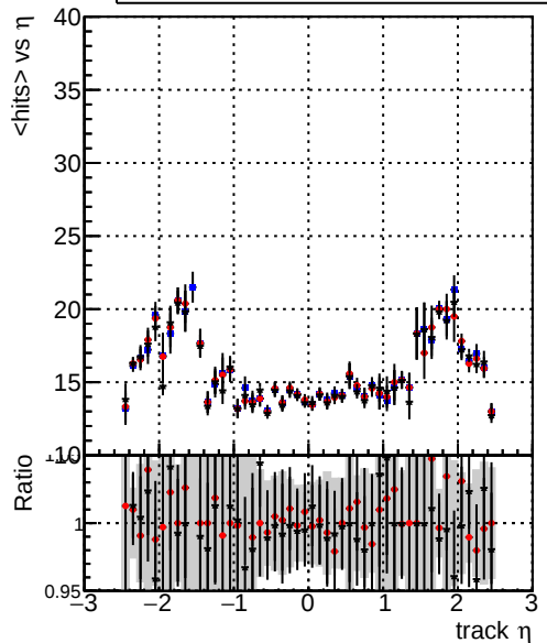
mean hits — DQM_TT_original — DQM_TT_mod_modelsdeep_truthfinal_reg_modelTEST-24 — DQM_TT_mod_modelsdeep_something3
