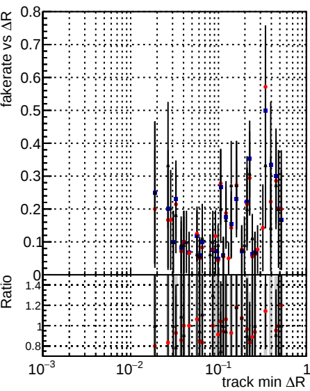
Legend: DQM TT original (blue dots), DQM TT mod modelsdeep_truthfinal_reg_modelTEST-24 (red dots), DQM TT mod modelsdeep_something3 (black dots)
