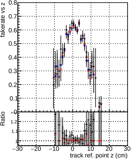
Fake rate vs vertpos Legend: DOM TT original DOM TT mod modelsdeep truthfinal_reg_modelTEST-24 DOM TT mod modelsdeep something3
