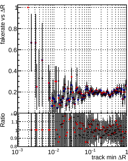
Legend: \Delta R (black dots), \Delta R (red dots), \Delta R (blue dots). Fake rate vs \Delta R (track, jet) Duplicates Rate vs \Delta R (track, jet) Pileup rate vs \Delta R (track, jet)
