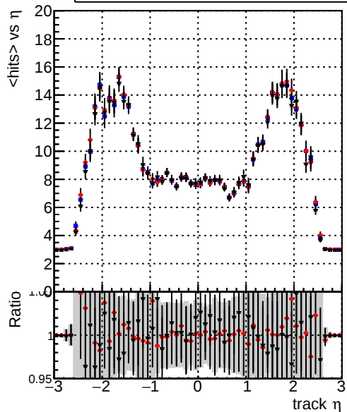
mean hit — DQM_TT_original — DQM_TT_mod_modelsdeep_truthfinal_reg_modelTEST-24 — DQM_TT_mod_modelsdeep_something3
