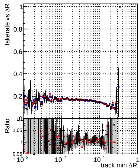
Legend for Fake rate vs \Delta R , Duplicates Rate vs \Delta R , and Pileup rate vs \Delta R : \blacksquare DQM TT original \bullet DQM TT mod modelsdeep_truthfinal_reg_modelTEST-24 \circ DQM TT mod modelsdeep_something3
