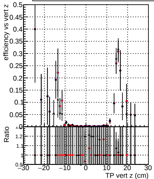
Efficiency vs. sim PV z — DQM_TT_original — DQM_TT_mod_modelsdeep_truthfinal_reg_modelTEST-24 — DQM_TT_mod_modelsdeep_something3
