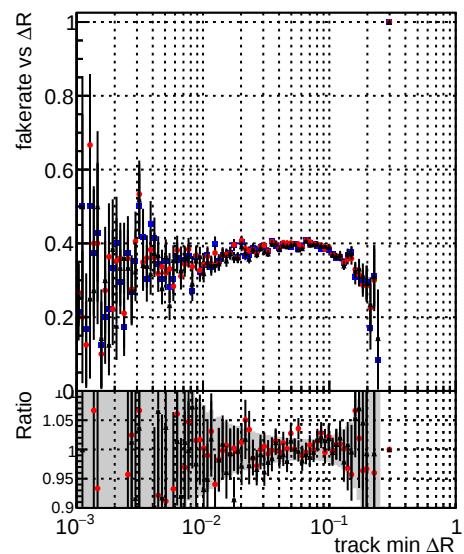
Legend for Fake rate vs \Delta R , Duplicates Rate vs \Delta R , and Pileup rate vs \Delta R : \blacksquare \Delta R original \bullet \Delta R mod modelsdeep_truthfinal_reg_modelTEST-24 \blacktriangledown \Delta R mod modelsdeep_something3
