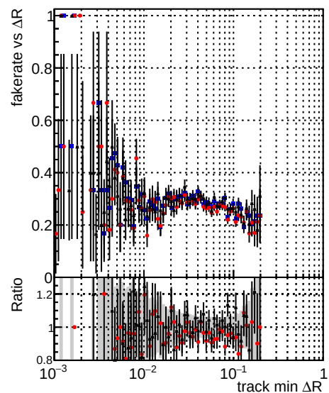
Fake rate vs \Delta R(\text{track, jet}) Legend: \square \Delta R(\text{track, jet}) original \square \Delta R(\text{track, jet}) mod modelsdeep_truthfinal_reg_modelTEST-24 \square \Delta R(\text{track, jet}) mod modelsdeep_something3
