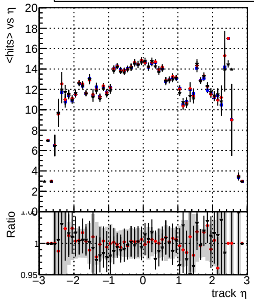
mean hits vs \eta — DQM_TT_original — DQM_TT_mod_modelsdeep_truthfinal_reg_modelTEST-24 — DQM_TT_mod_modelsdeep_something3
