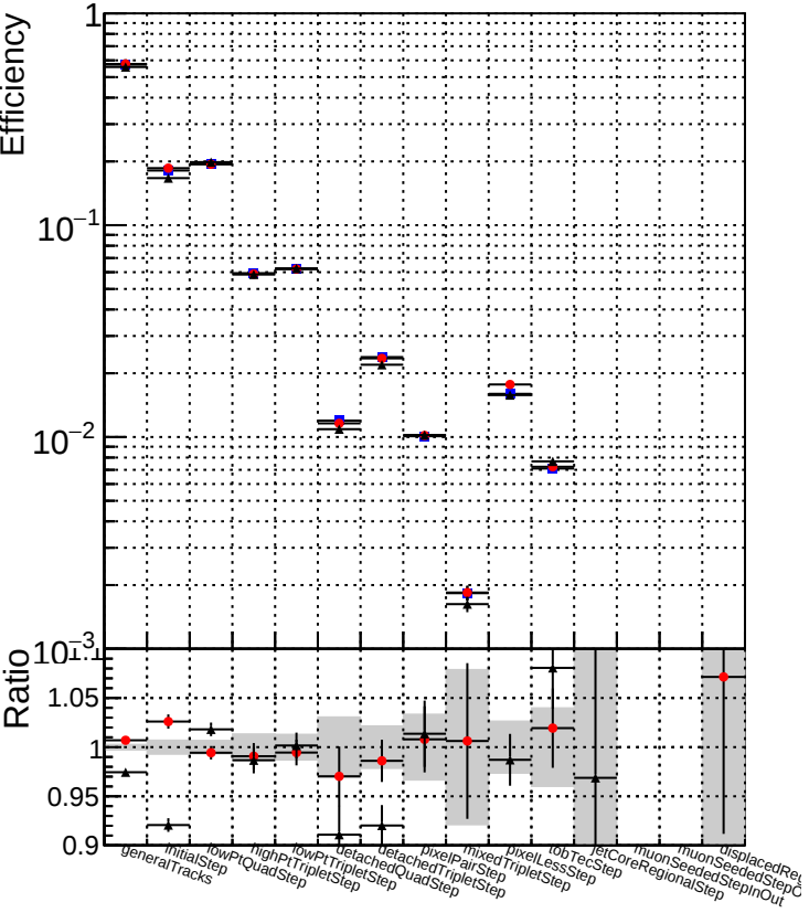
DQM_TT_original DQM_TT_mod_modelsdeep_truthfinal_reg_modelTEST-24 DQM_TT_mod_modelsdeep_somethingbetter
