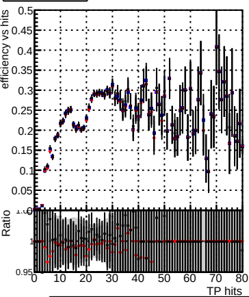
Efficiency vs hit Legend: DQM_TT_original DQM_TT_mod_modelsdeep_truthfinal_reg_modelTEST-24 DQM_TT_mod_modelsdeep_somethingbetter
