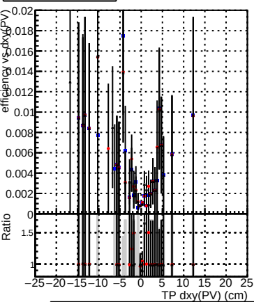
Efficiency vs Dxy(PV) Legend: DQM_TT_original (blue dots) DQM_TT_mod_modelsdeep_truthfinal_reg_modelTEST-24 (red dots) DQM_TT_mod_modelsdeep_somethingbetter (black dots)
