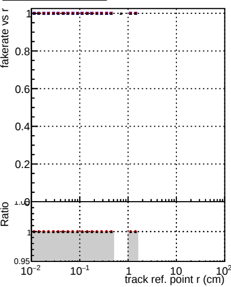
Fake rate vs v DOM TT original DOM TT mod modelsdeep_truthfinal_reg_modelTEST-24 DOM TT mod modelsdeep_somethingbetter
