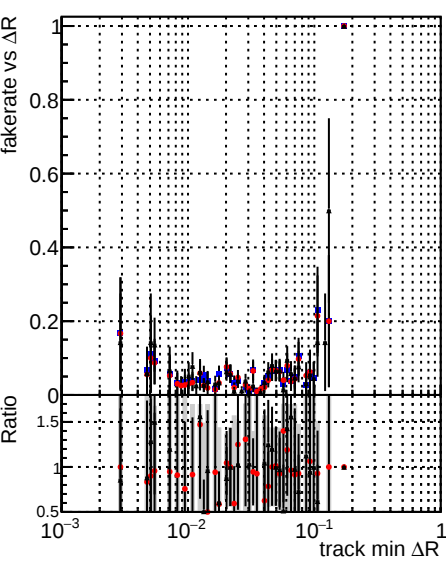
Fake rate vs ΔR(track, jet) DQM TT original DQM TT mod modelsdeep_truthfinal_reg_modelTEST-24 DQM TT mod modelsdeep_somethingbetter
