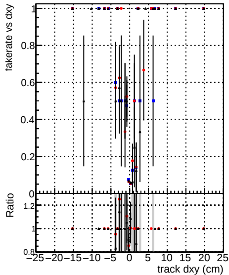
DOM TT original mod modelsdeep truthfinal reg. modelTEST-24 DOM TT mod modelsdeep somethingbetter
