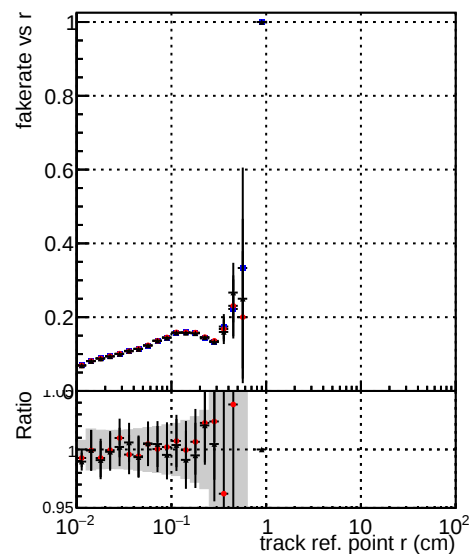
Fake rate vs v Legend: DOM TT original (blue circles) DOM TT mod modelsdeep_truthfinal_reg_modelTEST-24 (red circles) DOM TT mod modelsdeep_somethingbetter (black circles)
