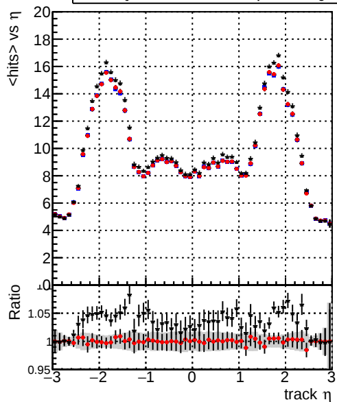
mean hits — DQM_TT_original — DQM_TT_mod_modelsdeep_truthfinal_reg_modelTEST-24 — DQM_TT_mod_modelsdeep_somethingbetter
