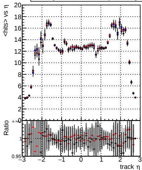
mean hits vs \eta Legend: DQM_TT_original (blue), DQM_TT_mod_modelsdeep_truthfinal_reg_modelTEST-24 (red), DQM_TT_mod_modelsdeep_somethingbetter (black)
