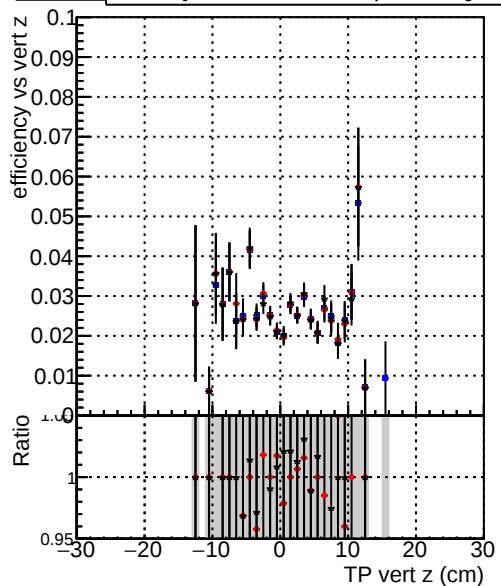
Efficiency vs. sim PV z — DQM_TT_original — DQM_TT_mod_modelsdeep_truthfinal_reg_modelTEST-24 — DQM_TT_mod_modelsdeep_somethingbetter
