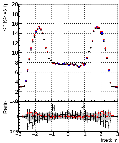
mean hits vs \eta — DQM_TT_original — DQM_TT_mod_modelsdeep_truthfinal_reg_modelTEST-24 — DQM_TT_mod_modelsdeep_somethingbetter
