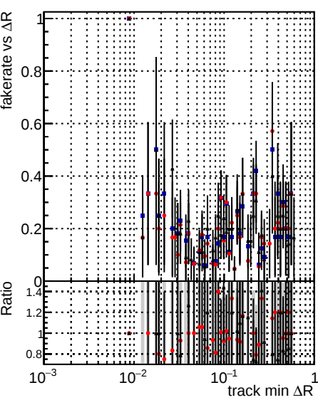
Fake rate vs ΔR(track, jet) Legend: DQM TT original DQM TT mod modelsdeep_truthfinal_reg_modelTEST-24 DQM TT mod modelsdeep_somethingbetter
