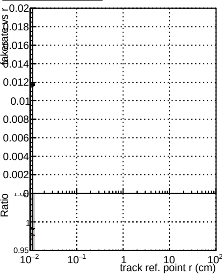
Legend: - DQM TT original (grey shaded region) - DQM TT mod modelsdeep truthfinal reg modelTEST-24 (blue dot) - DQM TT mod modelsdeep somethingbetter (red dot)
