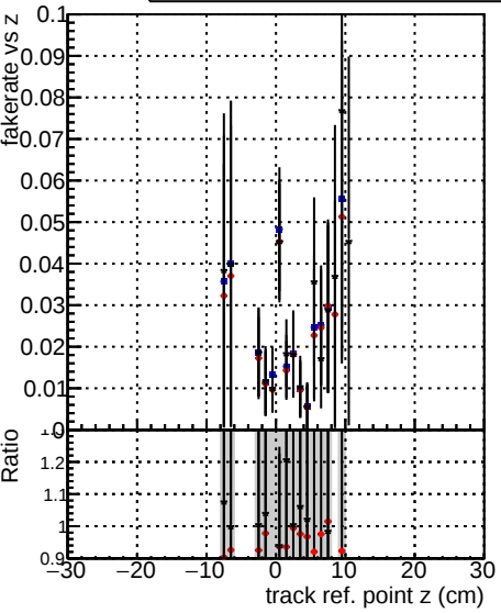
Fake rate vs verpos Legend: DQM TT original DQM TT mod modelsdeep truthfinal reg modelTEST-24 DQM TT mod modelsdeep somethingbetter
