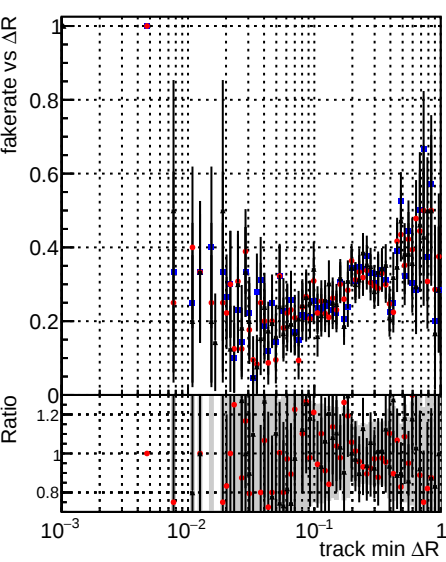
Legend: —●— DQM TT original —●— DQM TT mod modelsdeep_truthfinal_reg —●— DQM TT mod modelsdeep_truthfinal_reg modelTEST-24
