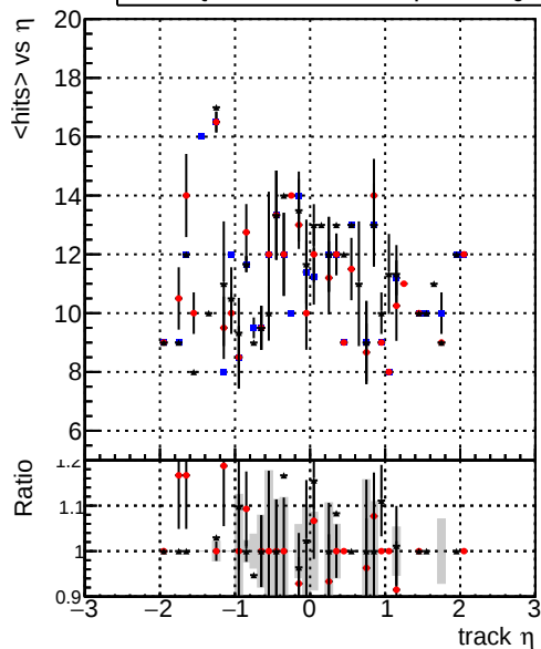
mean hit — DQM_TT_original — DQM_TT_mod_modelsdeep_truthfinal_reg_modelTEST-24 — DQM_TT_mod_modelsdeep_somethingbetter
