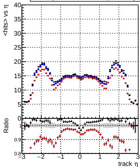
mean hit — DQM_TT_original — DQM_TT_mod_modelsdeep_truthfinal_reg_modelTEST-24 — DQM_TT_mod_modelsdeep_somethingbetter
