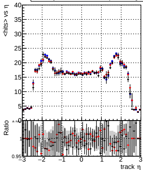
mean hits vs \eta Legend: DQM_TT_original (blue line), DQM_TT_mod_modelsdeep_truthfinal_reg_modelTEST-24 (red line), DQM_TT_mod_modelsdeep_somethingbetter (black line)
