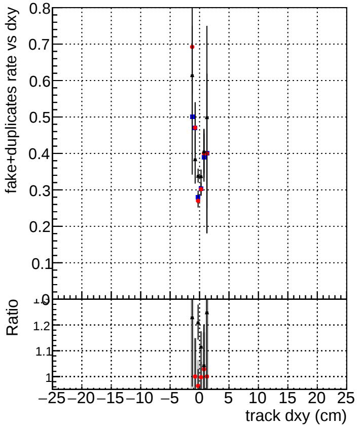
DQM_TT_original DQM_TT_mod_modelsdeep_truthfinal_reg_modelTEST-24 DQM_TT_mod_modelsdeep_somethingbetter
