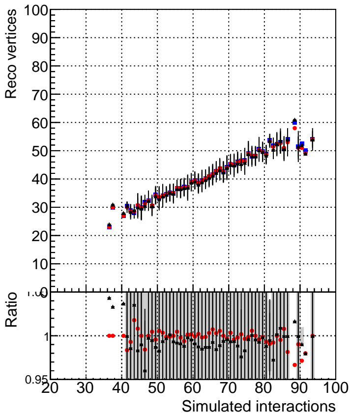
RecoVtx_vs_GenVtx
