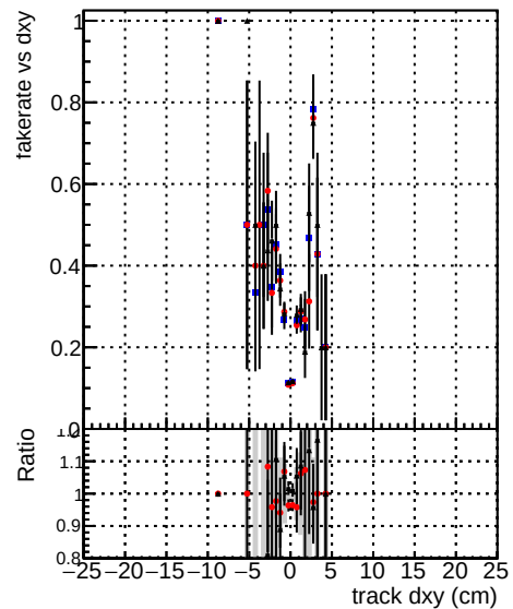
Fake rate vs d DOM TT original mod modelsdeep truthfinal reg. modelTEST-24 DOM TT mod modelsdeep somethingbetter
