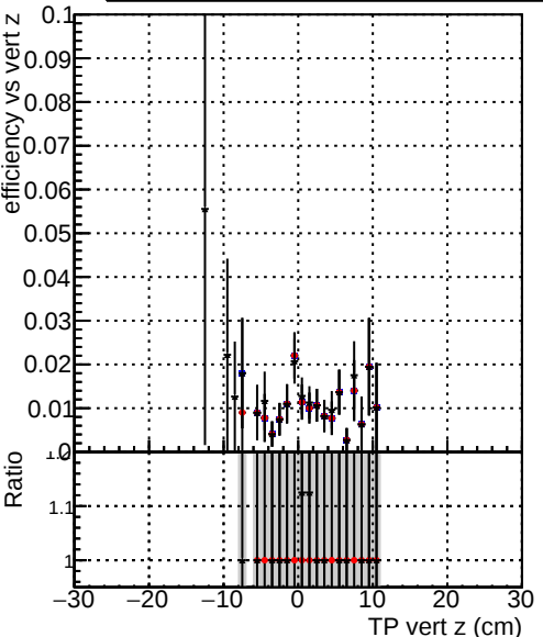
Efficiency vs TP vert z (cm) Legend: DQM_TT_original DQM_TT_mod_modelsdeep_truthfinal_reg_modelTEST-24 DQM_TT_mod_modelsdeep_somethingbetter
