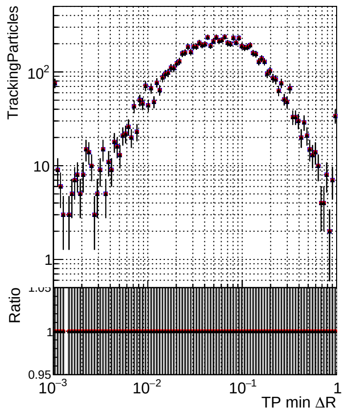
N of simulated tracks vs \Delta R (TP, jet) Legend: DQM TT original (blue square) DQM TT mod modelsdeep truthfinal_reg_modelTEST-24 (red circle) DQM TT mod modelsdeep somethingbetter (black triangle)
