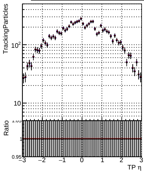
—•— DQM_TT_original —•— DQM_TT_mod_modelsdeep_truthfinal_reg_modelTEST-24 —•— DQM_TT_mod_modelsdeep_somethingbetter
