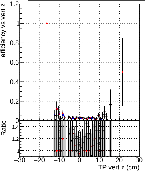
Efficiency vs vert z Legend: DQM_TT_original DQM_TT_mod_modelsdeep_truthfinal_reg_modelTEST-24 DQM_TT_mod_modelsdeep_somethingbetter
