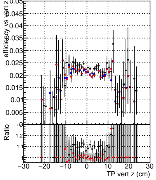
Efficiency vs vert z Legend: - DQM_TT_original (blue squares) - DQM_TT_mod_modelsdeep_truthfinal_reg_modelTEST-24 (red circles) - DQM_TT_mod_modelsdeep_somethingbetter (black crosses)
