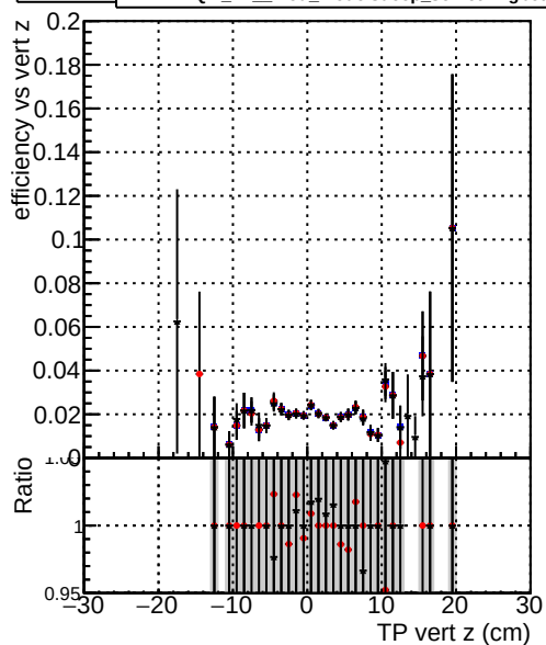
Efficiency —●— DQM TT mod modelsdeep_truthfinal_reg_modelTEST-24 —▲— DQM TT mod modelsdeep_somethingbetter
