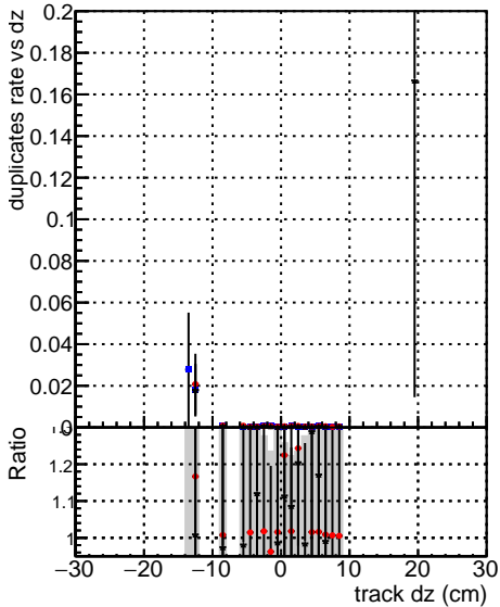
—●— DGM TT original —●— DGM TT mod —●— modelsdeep somethingbetter —●— truthfinal reg modelTEST-24
