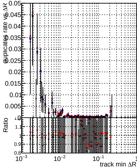
Legend for all plots: DQM TT original (black line with dots) DQM TT mod modelsdeep truthfinal reg modelTEST-24 (red line with dots) DQM TT mod modelsdeep somethingbetter (black line with dots)
