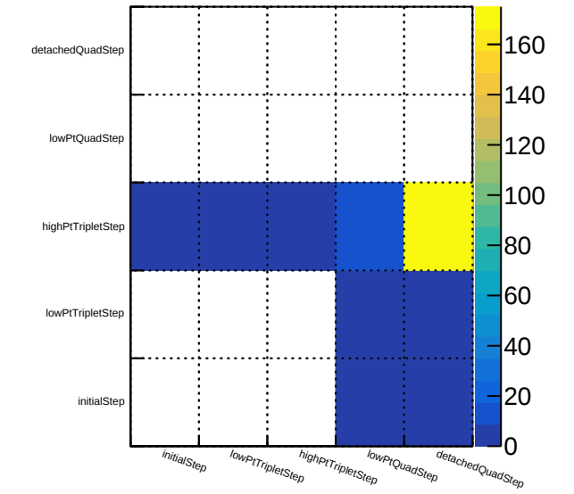
Duplicate tracks: originalAlgo vs originalAlgo
