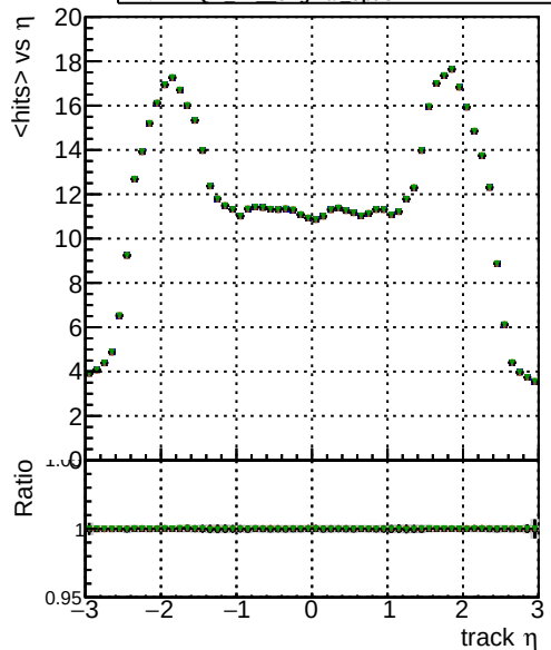
Legend for mean hits vs \eta : original RECO signal option2 signal option1 original option2 original option1 background
