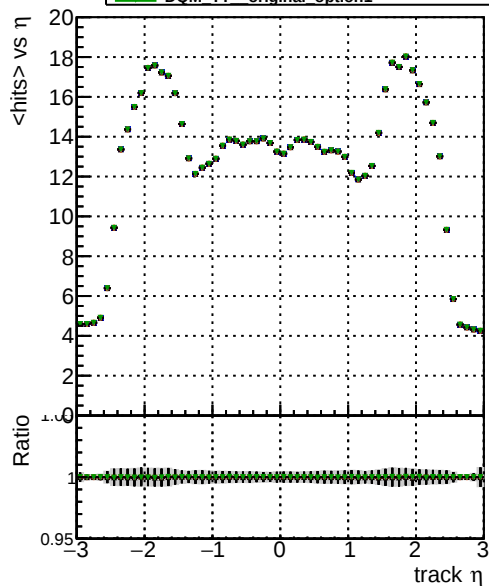
mean hit ■ BOM TT original REPO ■ BOM TT signal option0 ■ BOM TT signal option2 ■ BOM TT original option1 ■ BOM TT original option0
