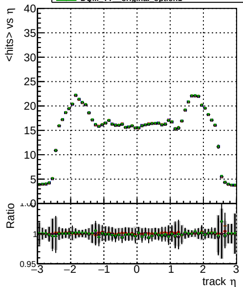
■ BQM TT original REPO ■ BQM TT signal option0 ■ BQM TT signal option2 ■ BQM TT signal option1 ■ BQM TT original option0 ■ BQM TT original option1 mean hits
