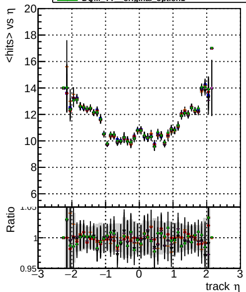
mean hit BOM TT original REPO BOM TT original option0 BOM TT original option1 BOM TT original option2 BOM TT original option3
