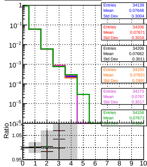
■ BQM TT original REPO ■ BQM TT signal option0 ■ BQM TT signal option2 ■ BQM TT original option2 ■ BQM TT original option1 mean hits
